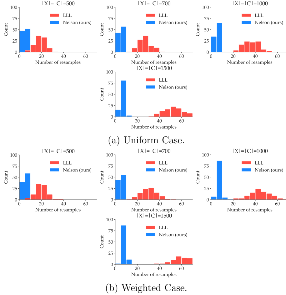
Figure 2.6. The distribution of resampling steps in the NELSON and Algorithmic-LLL [?]. Both of them get a valid sample within T_{tryouts} . NELSON takes much fewer resamples than Algorithmic-LLL because it resamples all the violated clauses at every iteration while Algorithmic-LLL only resamples one of them.
